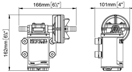
H 162 x L 166 x W 101 mm H 6 3/8" x L 6 1/2" x W 4"
