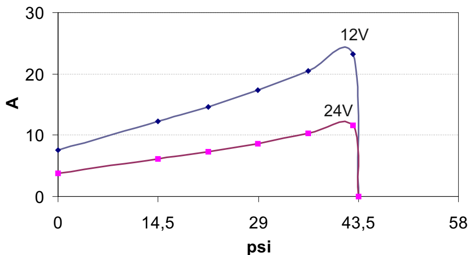
AMPERE-DRAW DIAGRAM
