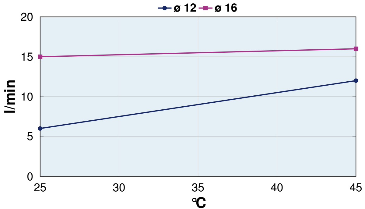
FLOW RATE
