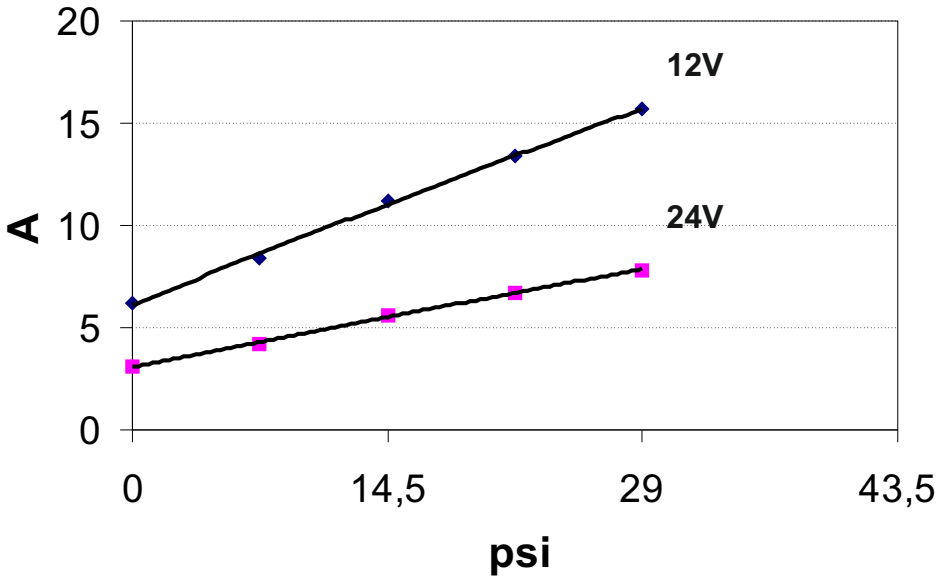
AMPERE-DRAW DIAGRAM
