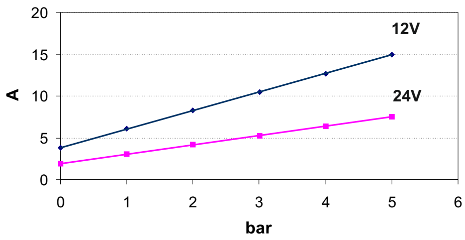
DIAGRAMME AMPERAGES AMPERE-DRAW DIAGRAM
